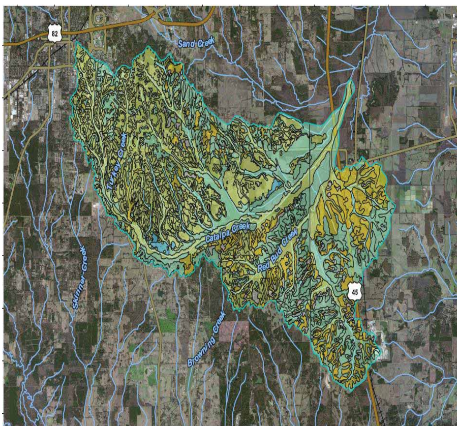
Figure 9.2.4. Available Water Capacity Classes for Soils in the Red Bud-Catalpa Creek Watershed.
